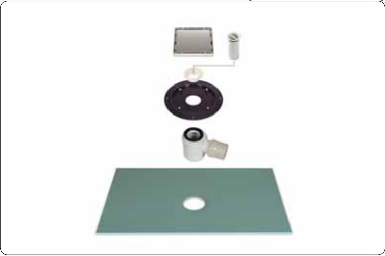
WET-DEC COMPONENTS
