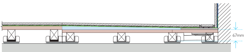
Typical details
